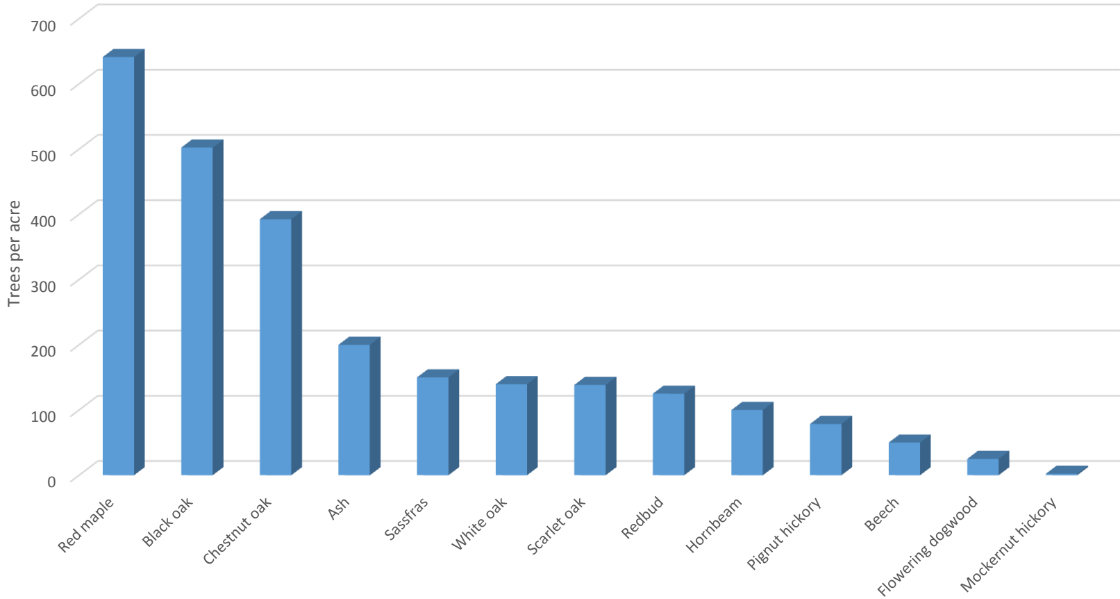
Area 9: Species composition by trees per acre
